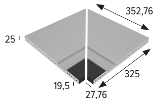
Esq. izda. nicho B33 SPORT B33 SPORT niche left corner
