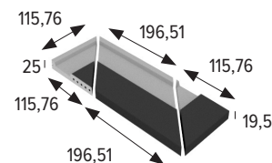
Esq. dcha. nicho B33 SPORT B33 SPORT niche right corner
