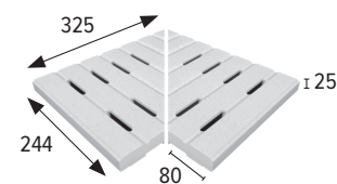
Esquina rejilla Corner grid **
