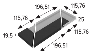
Esq. izda. nicho B33 SPORT B33 SPORT niche left corner
