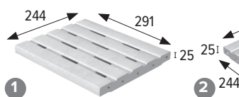
Rejilla monocomp. ranurada Monocompact grooved grid**
