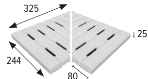
Esquina rejilla Corner grid **
