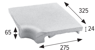
Remate esquina interior Internal corner
