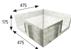
Pieza esquina interior Internal corner piece
