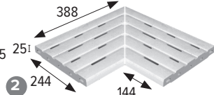
Esquina rejilla Corner grid
