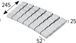
Rejilla flexible ranurada Grooved Flexible grid *
