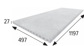
Borde monocompact 120 Monocompact edge 120
