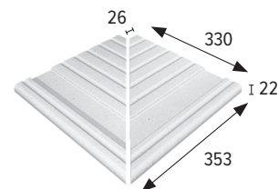
Esquina rejilla Corner grid **
