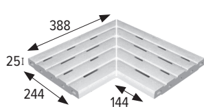
Esquina rejilla Corner grid
