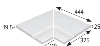
Esquina rejilla Corner grid
